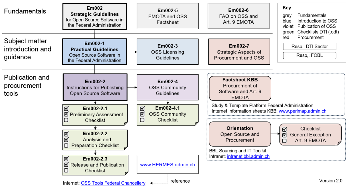
Figure 1: Overview of OSS tools
